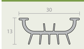
RP304Si silicon rubber (SE)
