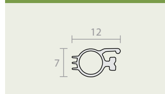
RP394Si LG silicon rubber (SE)
