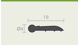
RP303 solid EPDM
