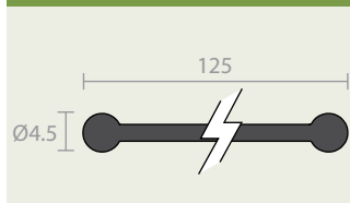
RP394Si GR silicon rubber (SE)
