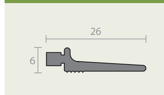
RP371Si GR silicon rubber (SE)
