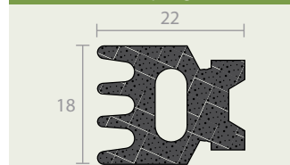
RP347Si silicon rubber (SE)
